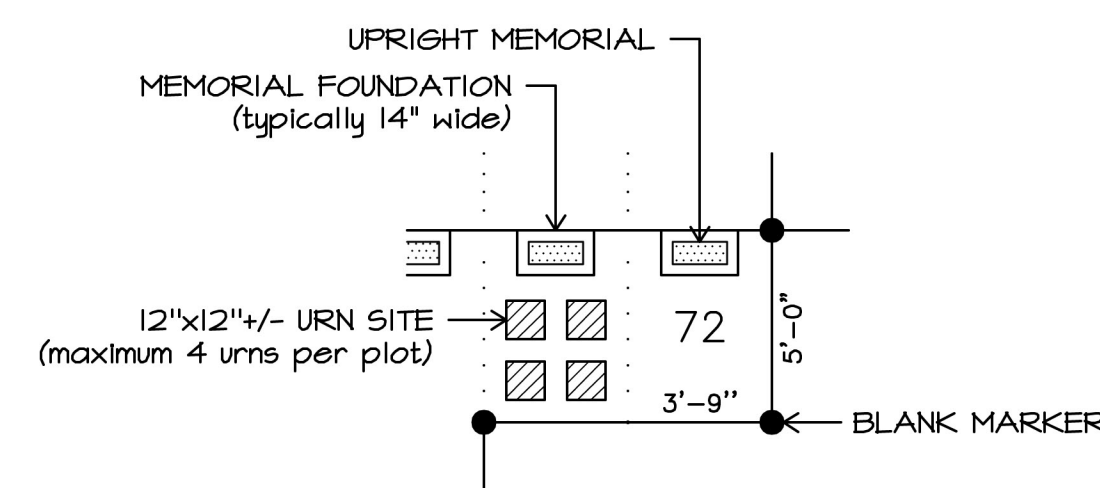
PLOT SIZE: 3'-9" x 5'-0" SCALE : 1"=5'
